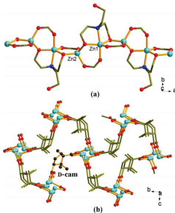
Figure 2. View of the 1D chiral connectivity [Zn( \Lambda -Zn(Htea))] n from achiral sources (a) and the 3D chiral connectivity [Zn(D-cam)] n from the enantiopure camphorates (b) in 1DA .
