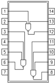
7410 Triple 3-Input NAND Gate
