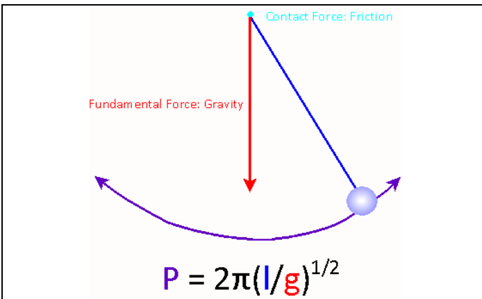
Diagram illustrating how both contact and fundamental forces operate in pendulums. Since all contact forces result from fundamental forces acting on objects, the pendulum’s swing as well as the contact pressure that results in the drag at the arm pivot result from the fundamental force of gravitation (in red). The contact force, friction (in light blue), operates at the pendulum arm pivot resulting from the surface drag during the swing of the pendulum.
