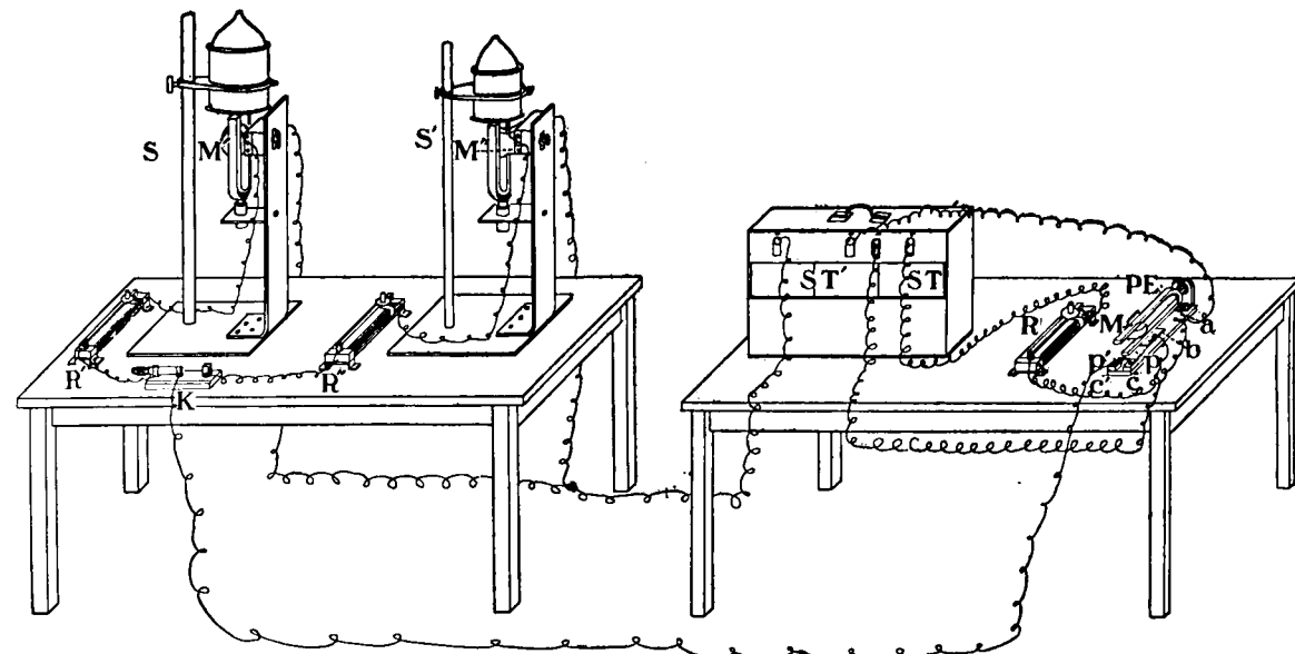
FIG. 11. JOHNSON'S MODIFICATION OF HELMHOLTZ'S SYSTEM OF TANDEM-DRIVEN FORKS
